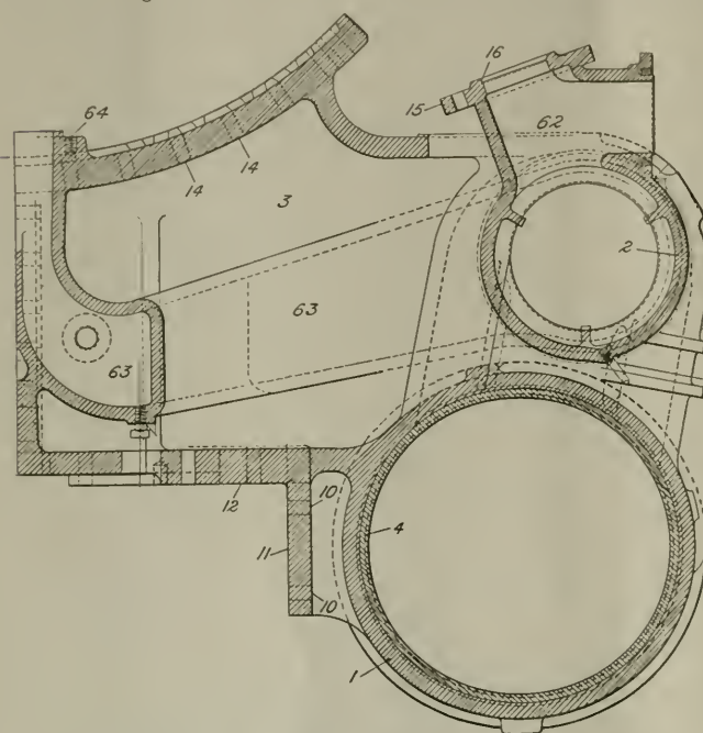
CROSS SECTION OF CYLINDERS, SADDLE AND STEAM CHEST
